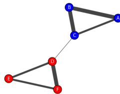
Figure 5.5: Example of a weighted graph.
