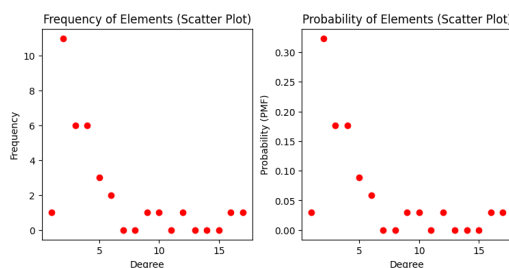
Figure 5.6: Frequencies and PMF for the degree distribution of the “Zachary Karate Club” network.
