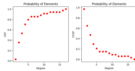
Figure 5.7: CDF and CCDF for the degree distribution of the “Zachary Karate Club” network.
