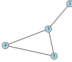
Figure 5.3: Example of a closed neighbourhood within a graph.
