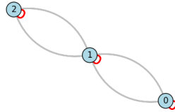
Figure 5.4: Example of a graph that is not simple.
